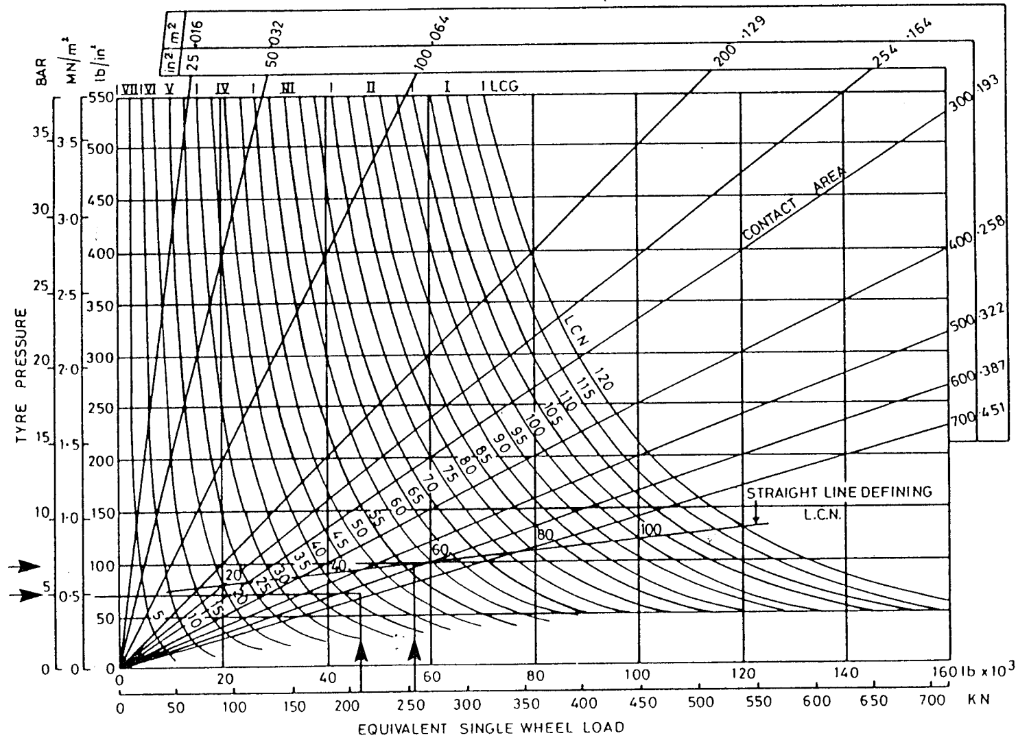
FIG.3 LCN AND LCG IN TERMS OF ESWL TYRE PRESSURE AND TYRE CONTACT AREA
